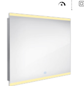
LED mirror 900 x 700 With touch sensor. Possibility of setting the color temperature 2700K - 6000K. Output 26W. Aluminium frame.
